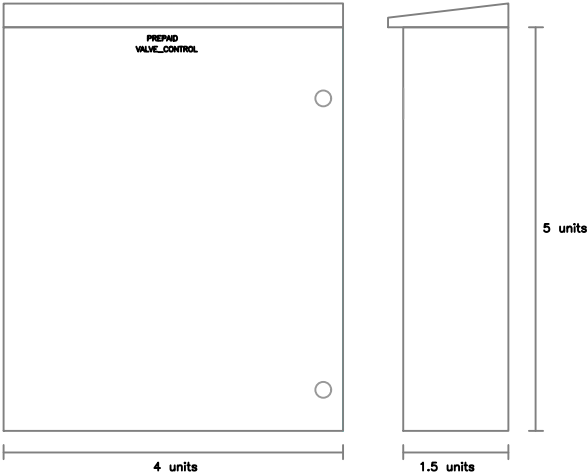
OUTER VIEW SABELCO IP65 ENCLOSURE
